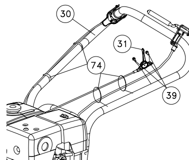
Good routing
