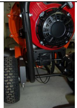
Bad routing
